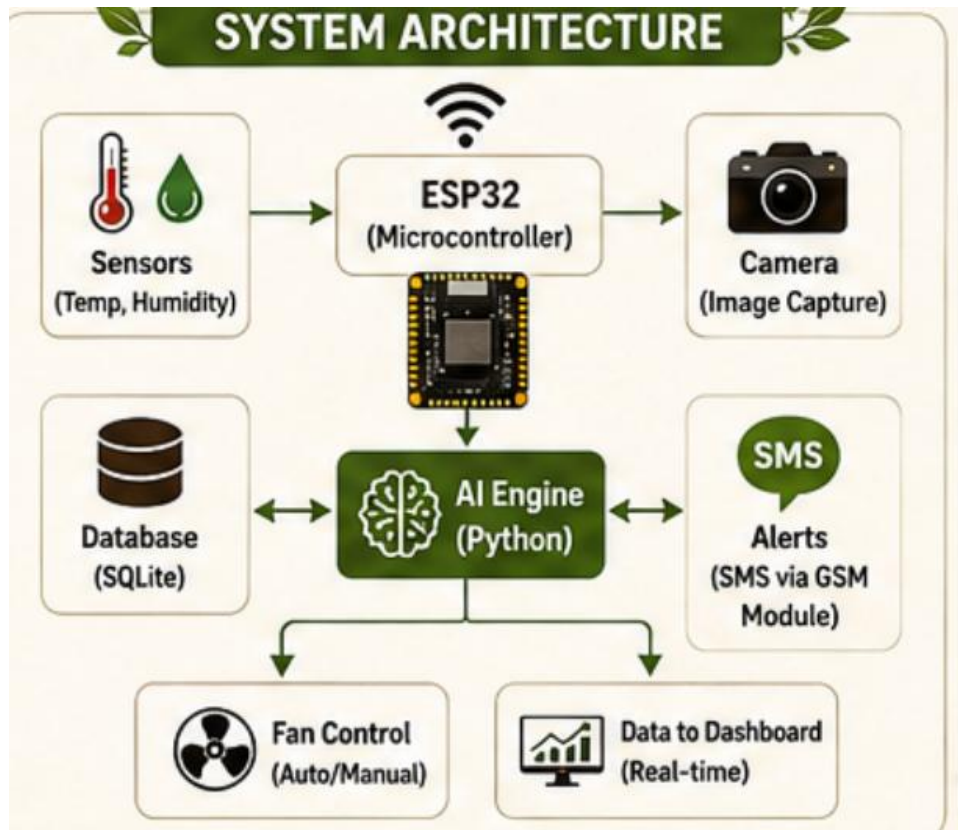
Fig. 3.5 — System Architectural Diagram
