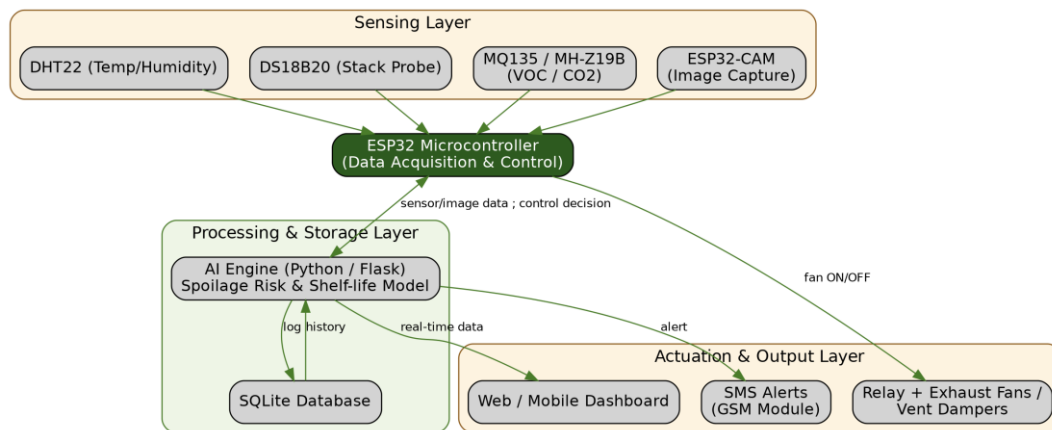
Fig. 4.1 — Block Diagram of the Project
