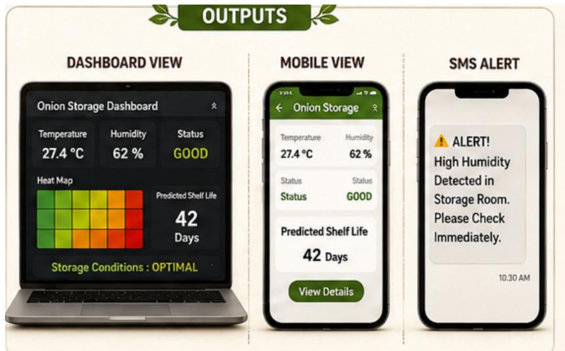
Fig. 5.1 — Proposed dashboard, mobile view and SMS alert interfaces
